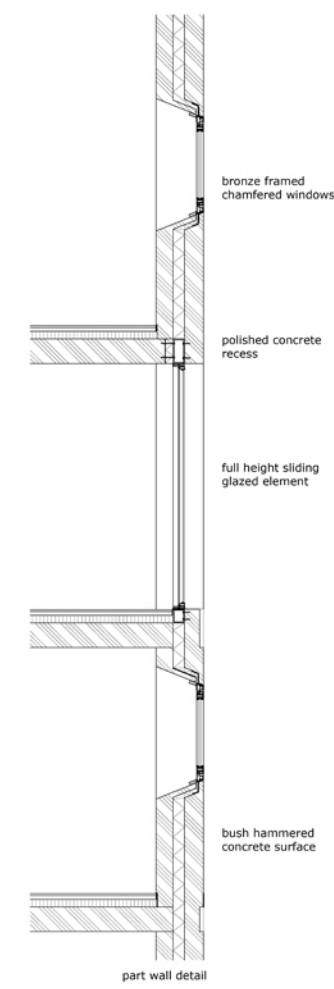
part wall detail
