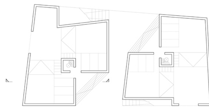
ground floor plan 1:200
