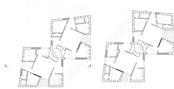
third floor plan 1:200
