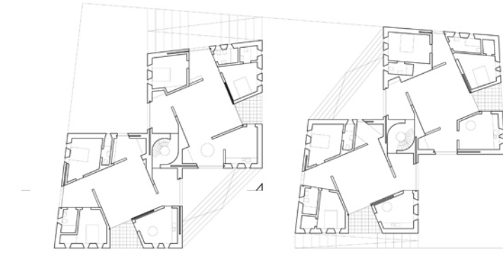
first floor plan 1:200
