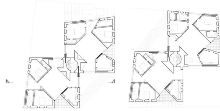
second floor plan 1:200
